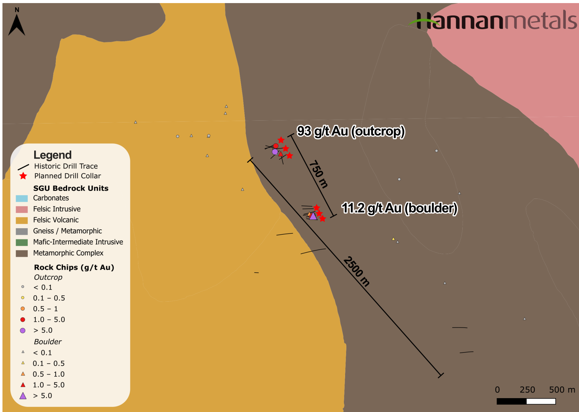
Figure 3: Geology map of the Stavaträsk project showing planned drilling, historic drilling and surface geochemistry.
